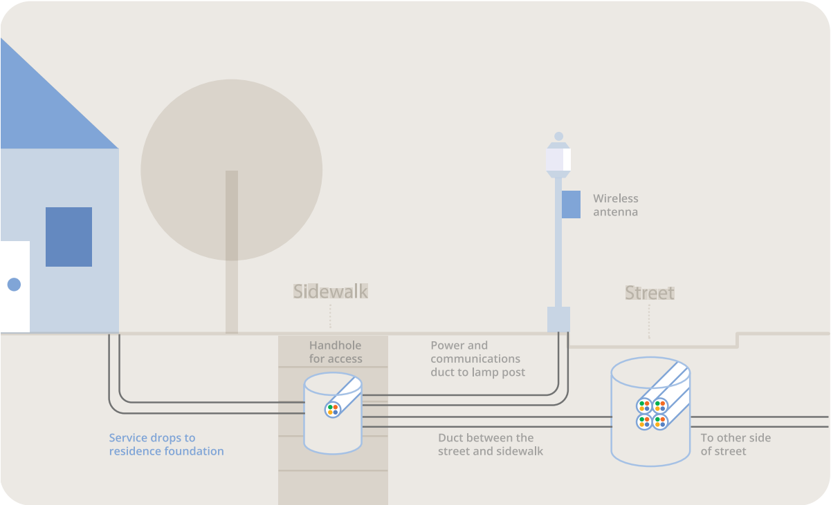
FIGURE 13: LONG-TERM CONDUIT INSTALLATION STRATEGY
