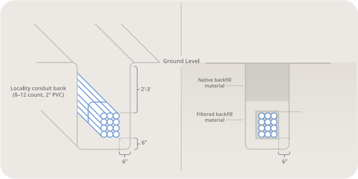
FIGURE 15: UNDERGROUND CONDUIT BANK FOR MULTIPLE USERS
