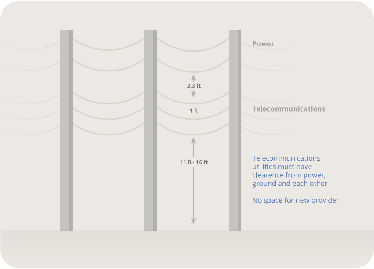
FIGURE 17: BASIC POLE DIAGRAM FOR MAKE-READY
