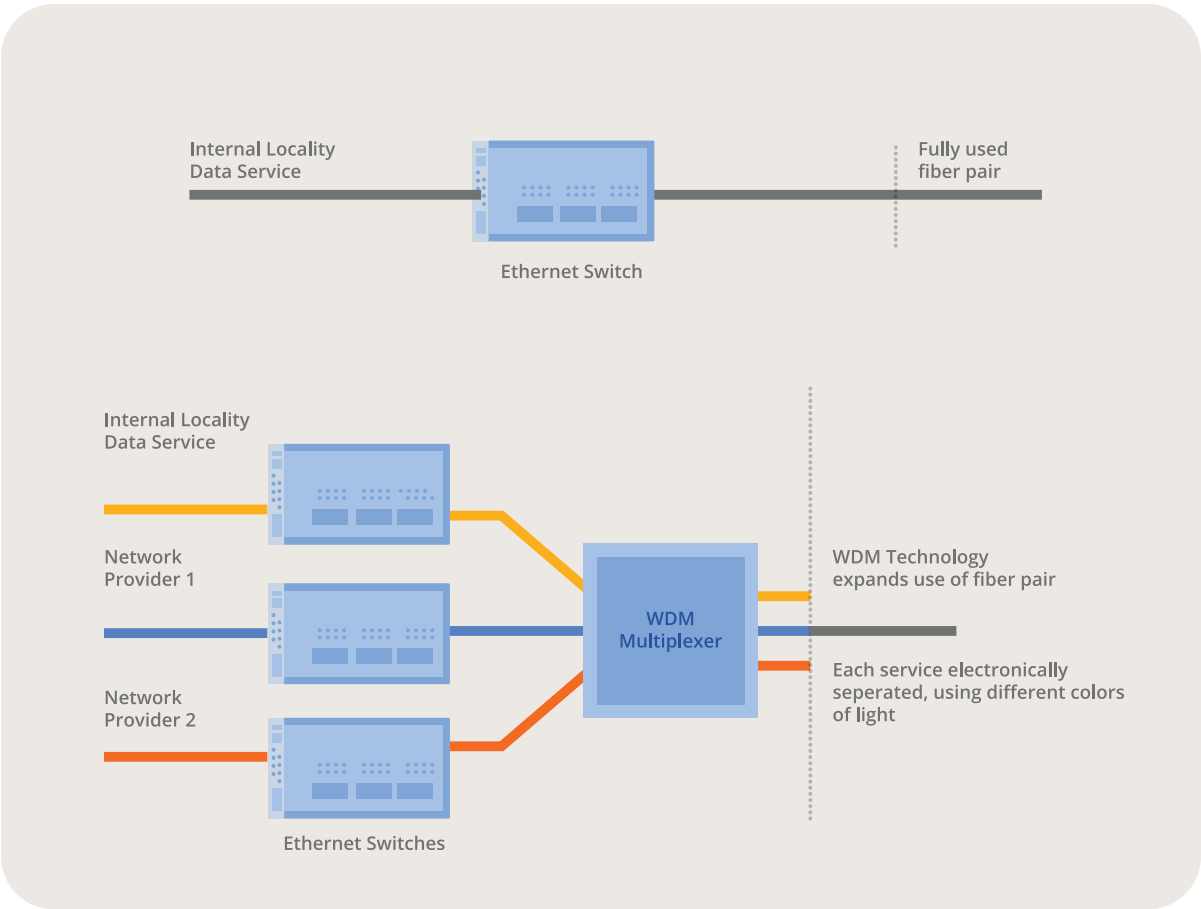
FIGURE 6: USE OF DWDM TO EXPAND FIBER CAPACITY
